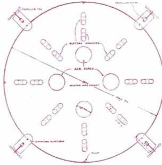
PLAN OF BASE OR PITHA
